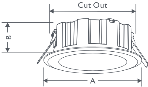
Lum. Dimensions (Unit:mm)
